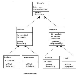
Figure 1: Vehicle Classification with Class Inheritance
