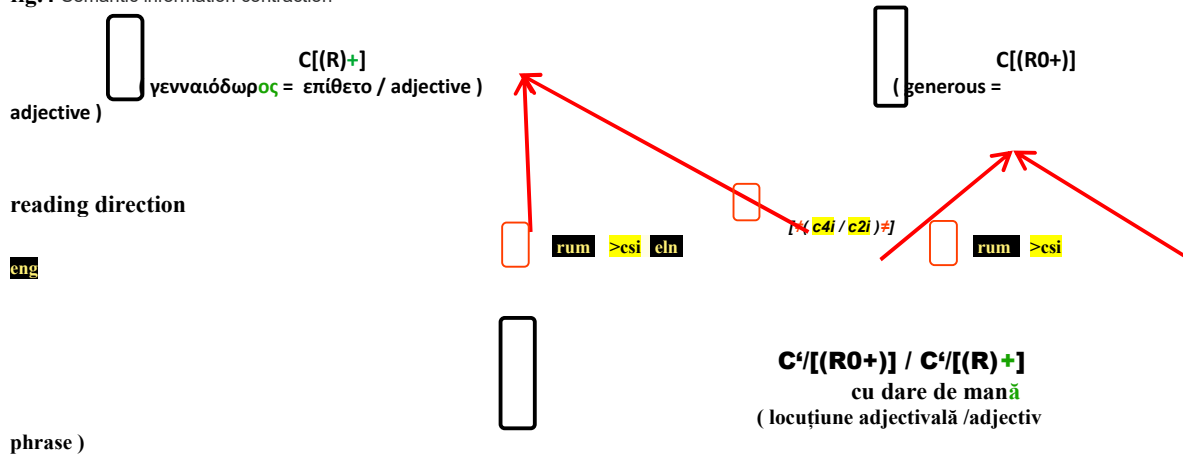
fig.4 Semantic information contraction
