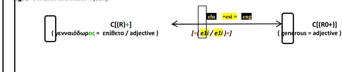
fig. 5 Semantic information equality
